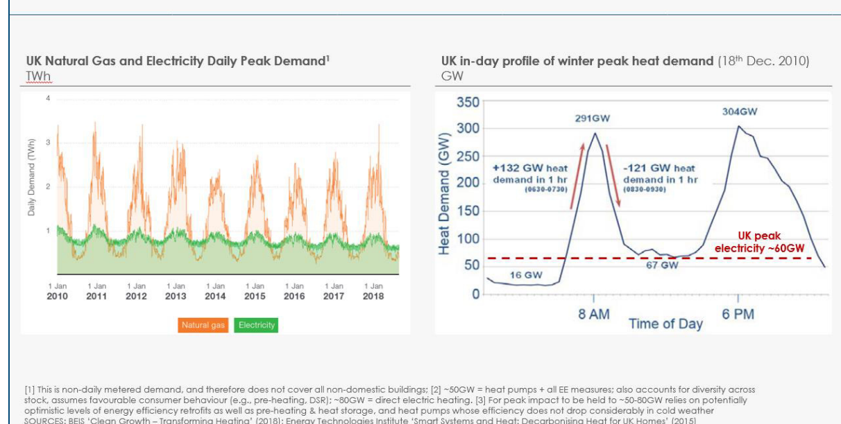
Exhibit 6: volumes of energy for heat – daily total, within-day fluctuations [UK example]
